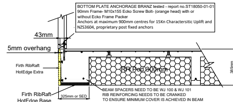
② 300mm FIRTH RIBRAFT POLYPOD 90mm WALL FRAME HOTEDGE EXTRA & HOTEDGE BASE FIRTH RAFTMIX 20 OR 25MPa
