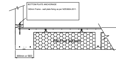
⑧ 300mm FIRTH RIBRAFT POLYPOD 140mm WALL FRAME FIRTH RAFTMIX 20 OR 25MPa
