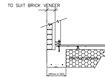
⑫ 300mm FIRTH RIBRAFT POLYPOD BRICK VENEER FIRTH RAFTMIX 20 OR 25MPa
