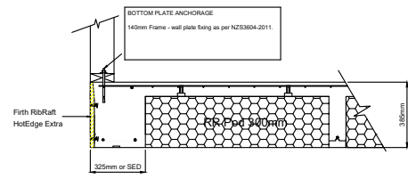
⑤ 300mm FIRTH RIBRAFT POLYPOD 140mm WALL FRAME HOTEDGE EXTRA FIRTH RAFTMIX 20 OR 25MPa
