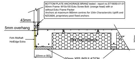
③ 300mm FIRTH RIBRAFT POLYPOD 90mm WALL FRAME HOTEDGE EXTRA WITH XPS INSULATION IN BEAMS & RIBS FIRTH RAFTMIX 20 OR 25MPa
