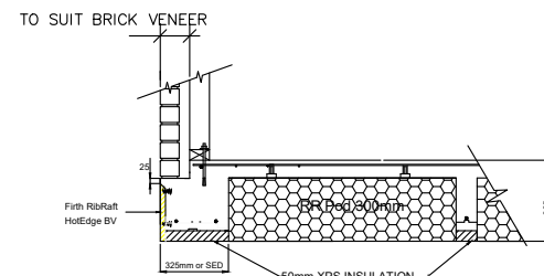
⑪ 300mm FIRTH RIBRAFT POLYPOD BRICK VENEER HOTEDGE WITH XPS INSULATION IN BEAMS & RIBS FIRTH RAFTMIX 20 OR 25MPa
