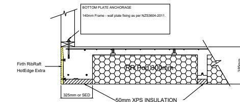
⑦ 300mm FIRTH RIBRAFT POLYPOD 140mm WALL FRAME HOTEDGE EXTRA WITH XPS INSULATION IN BEAMS & RIBS FIRTH RAFTMIX 20 OR 25MPa
